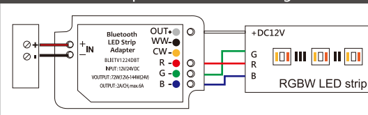
3CH Bluetooth adapter connected to the light bar
