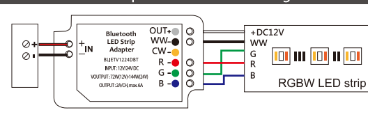
4CH Bluetooth adapter connected to the light bar
