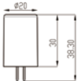
□金:G4.0
