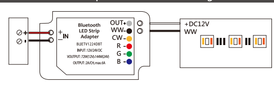
1CH Bluetooth adapter connected to the light bar
