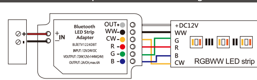
5CH Bluetooth adapter connected to the light bar
