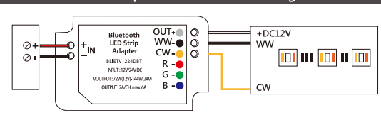
2CH Bluetooth adapter connected to the light bar
